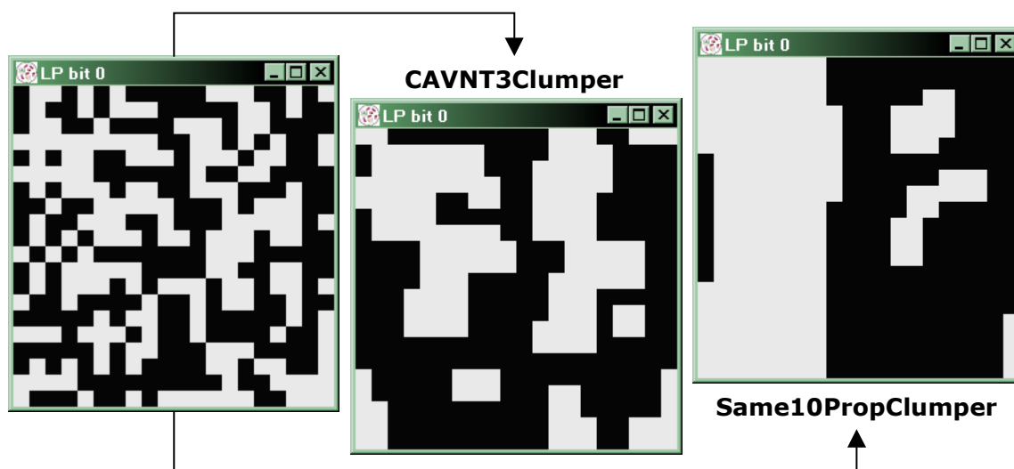
Figure 5 — The effect of the two clumpers. Left : Original Biophysical Properties generated at random, which was used as the initial state for both clumpers shown. Middle : CAVNT3Clumper after 6 cycles (the 7th having no effect). Right : Same10PropClumper.
