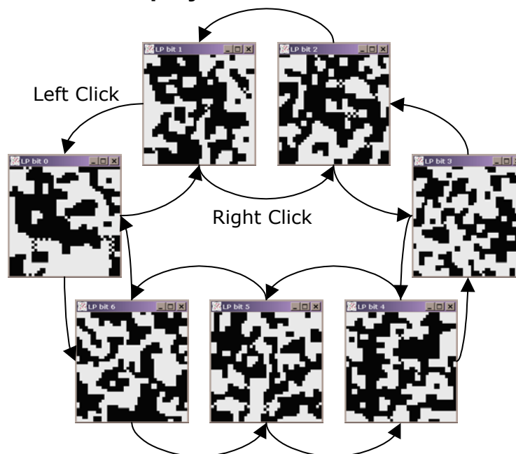
Figure 19 — The Biophysical Properties raster, which is displayed if the showLPBitStringRaster parameter is set to 1 in the observer file. This shows the spatial distribution of one bit of the Biophysical Properties at a time. Black is used for a value of 1, white for 0. The bits are numbered from 0 to one less than the Biophysical Properties bitstring length. Left-clicking decreases the number of the bit displayed, and right-clicking causes it to increase, wrapping round from the 0th bit to the maximum bit and vice versa. The bit displayed is shown in the title bar of the window.
