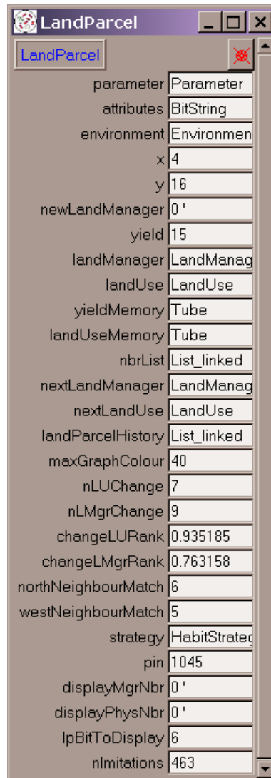
Figure 15 — The Land Parcel window obtained by right-clicking on a cell in the Land Manager raster.
