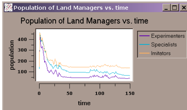
Figure 20 — Time-series graph showing the number of members in each of three Subpopulations during the course of a run.
