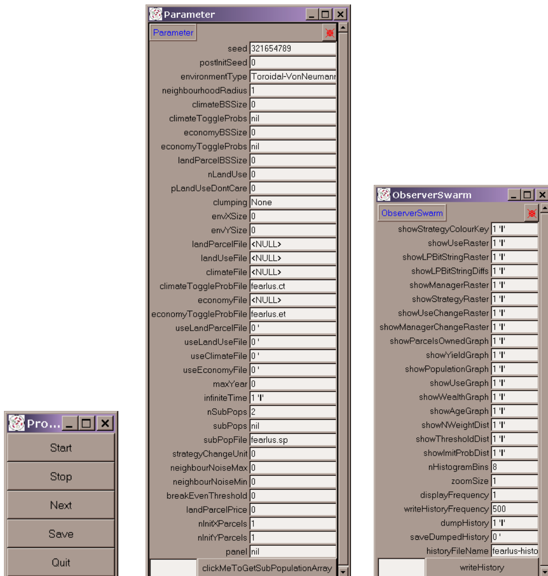
Figure 8 — The three windows that pop up on starting model0-6-4. The illustration here shows what appears if you start model0-6-4 without any parameter file specified using the -p or -o flags. In the parameter window, the user has entered ‘2’ in the box against the ‘nSubPops’ parameter.
